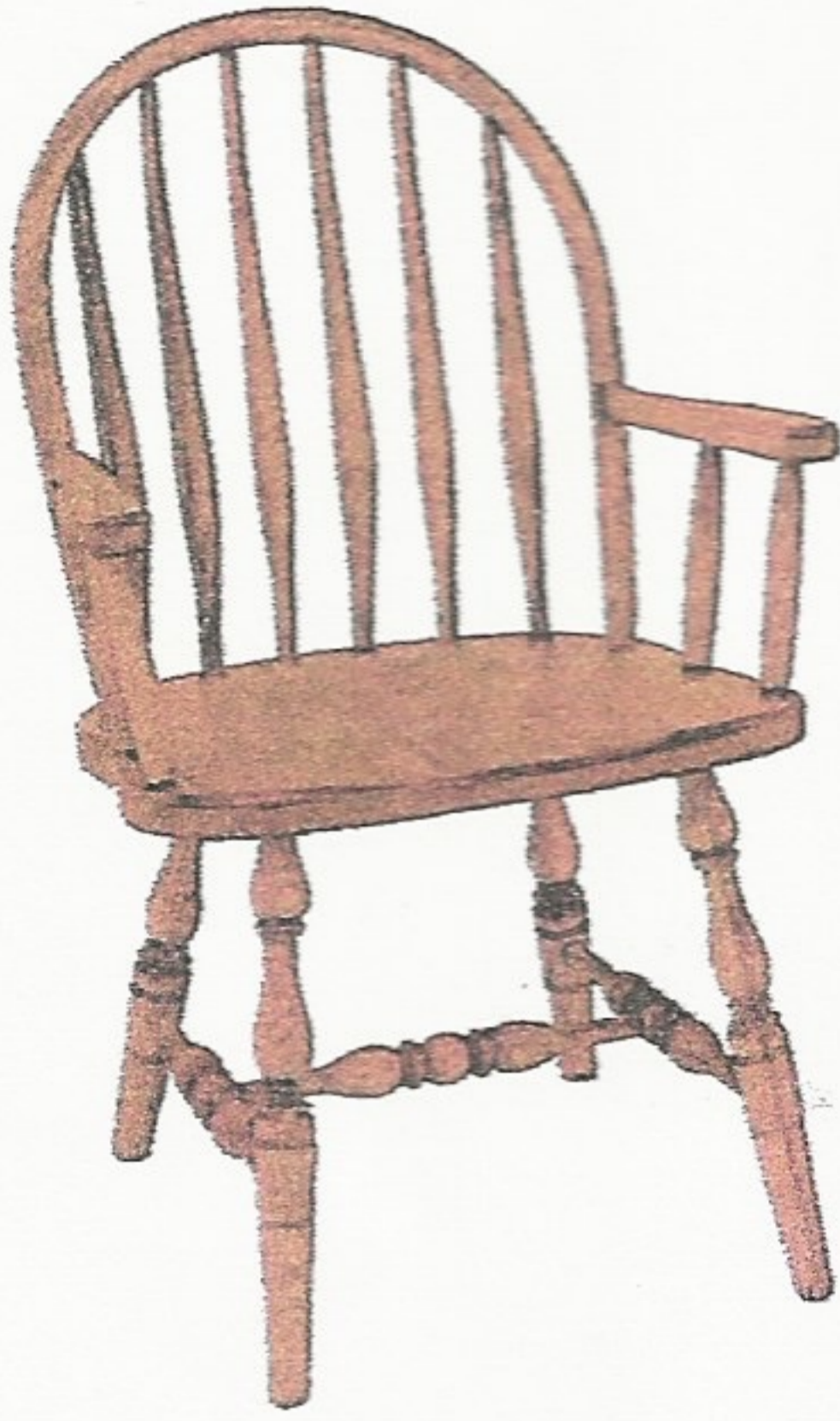
Low Bent Feather Arm 36½" h x 17¾" d x 22½" w Arm Height: 26"
